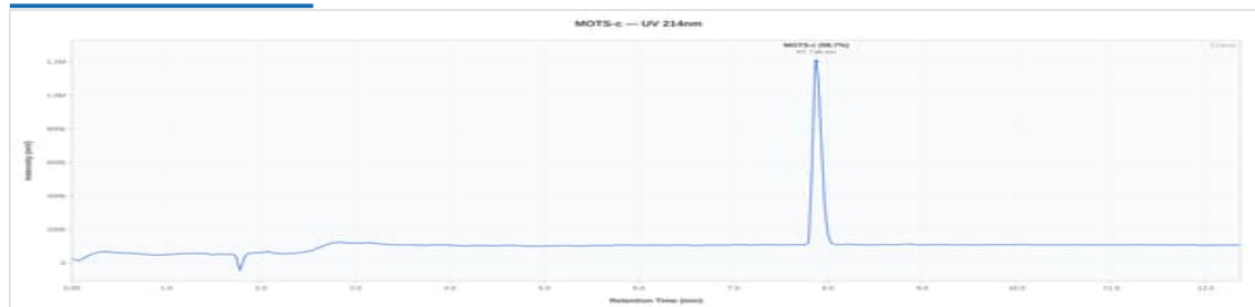
MOTS-C 10mg - 052826-MOT-B: UV Chromatogram
