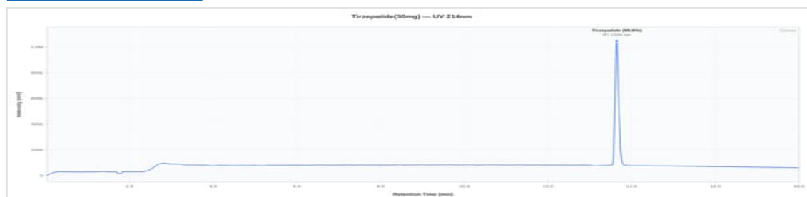
Tirzepatide 30mg - 051926-T30-8: UV Chromatogram
