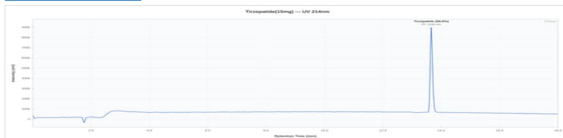
Tirzepatide 15mg - 051926-T15-C: UV Chromatogram
